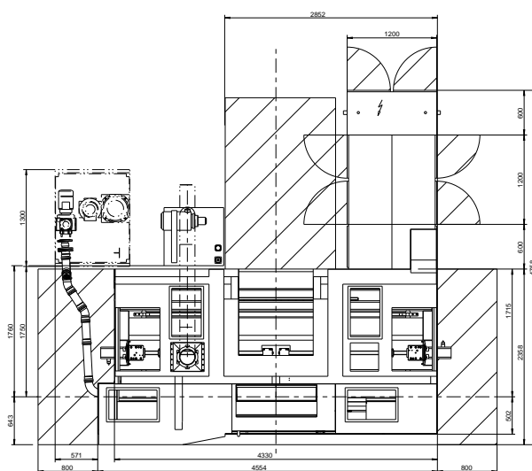
Layout CamGrind L2
