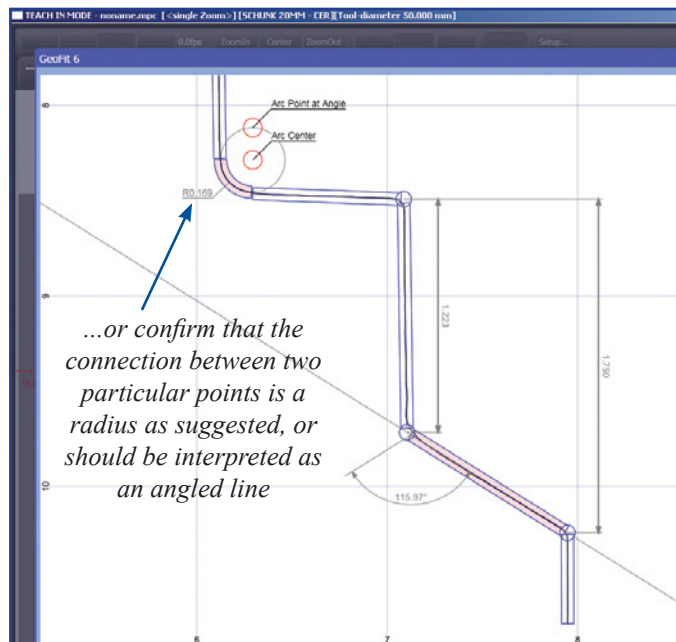
Easy Check's profile editor lets you quickly define the measurements you want. For example, you can tell the software to measure multiple step lengths from the same starting point...
