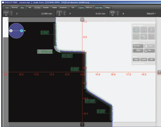
Easy Check scans the region you select in detail and automatically detects the profile
